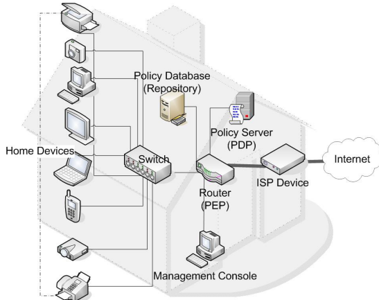
Fig. 4: PBTM in HAN.
