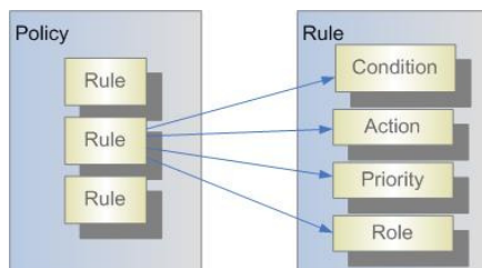
Fig. 1: Policy anatomy.
